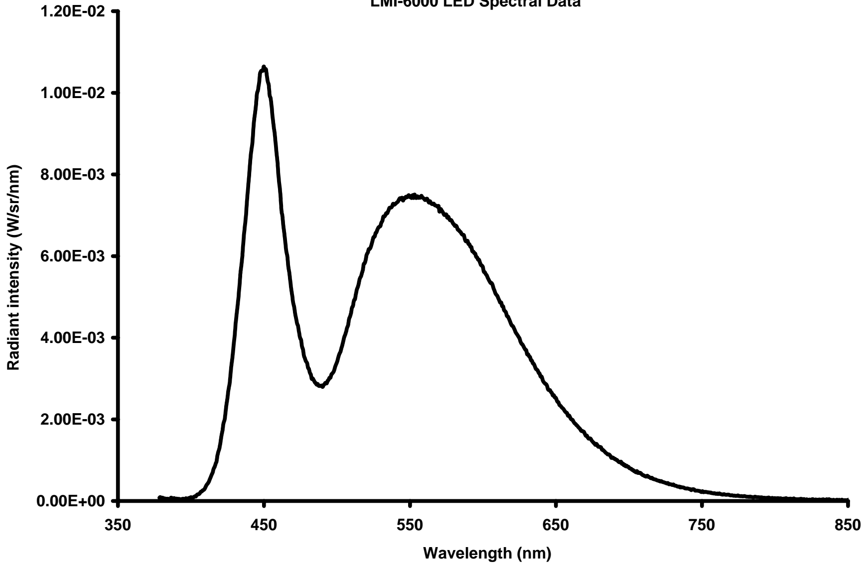
LMI-6000 LED Spectral Data
